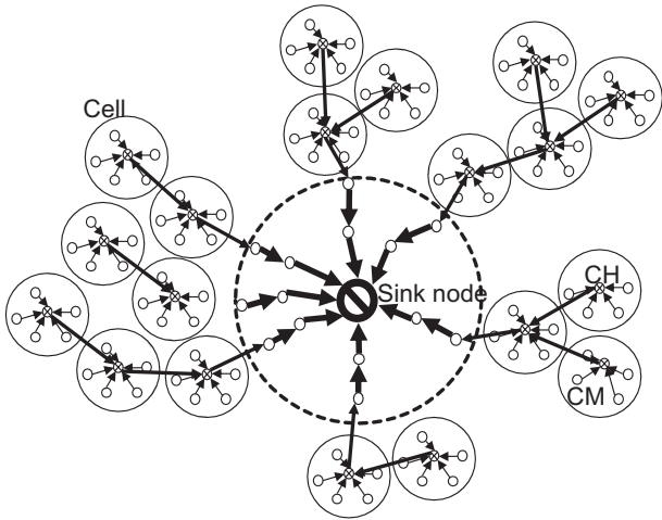
Fig. 5. Hybrid multi-hop routing.
