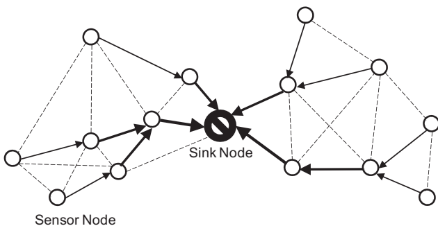
Fig. 1. Flat multi-hop routing.
