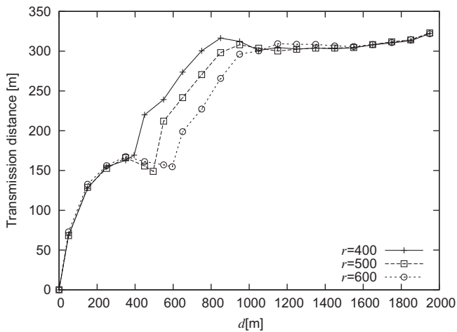
(a) Transmission distance in each node.
