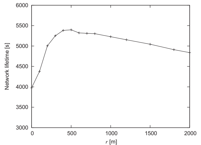
(a) Effect of hybrid boundary on network lifetime.
