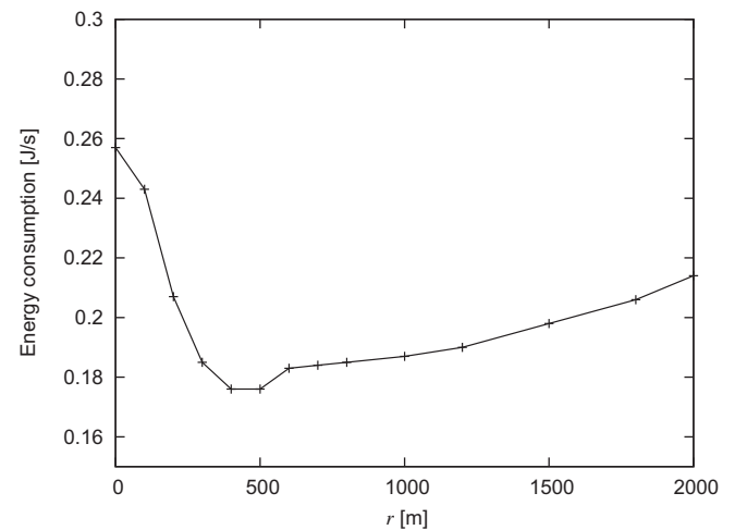
(b) Effect of hybrid boundary on energy consumption in the hotspot.
